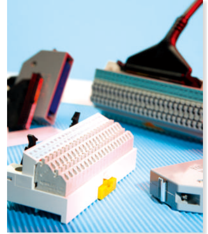
PLC Terminal terminal module Series Type CXT-W ... Certifications CE
